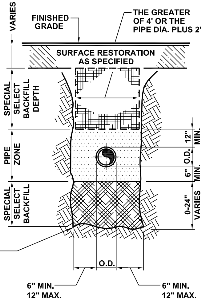
SPECIAL BACKFILL DETAIL A
