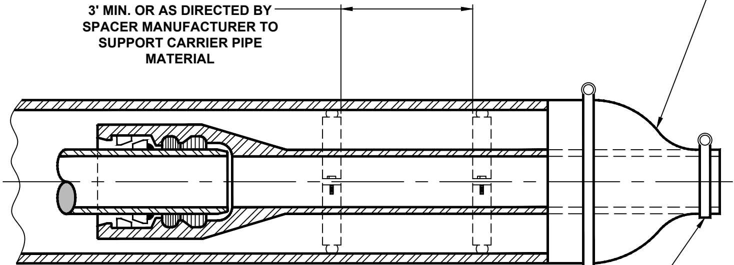
SECTION B
